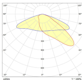
L2 Lens
