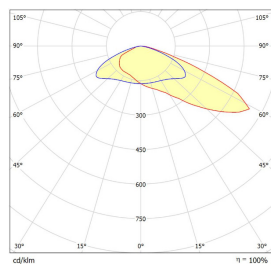
L1 Lens
