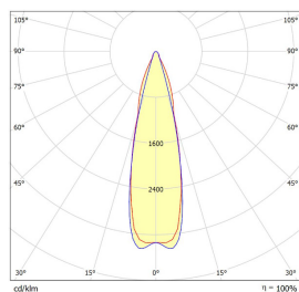
L8 Lens
