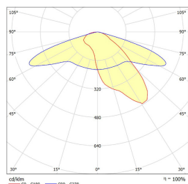
L6 Lens
