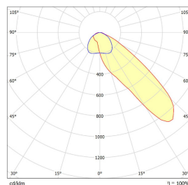
L4 Lens
