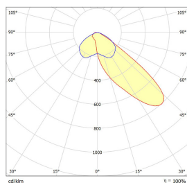
L3 Lens
