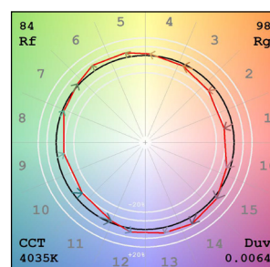
TM-30 Spectrum
