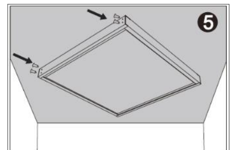
5. Re-attach the side to the frame with Screw A
