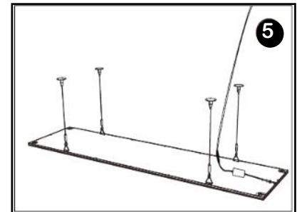
5. Attach hooks to suspension points on panel as shown above
