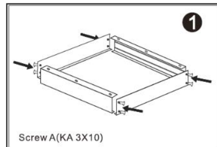
1. Assemble the four sides with Screw A to form a rectangular frame
