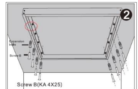
2. Mount the rectangular frame to the ceiling
