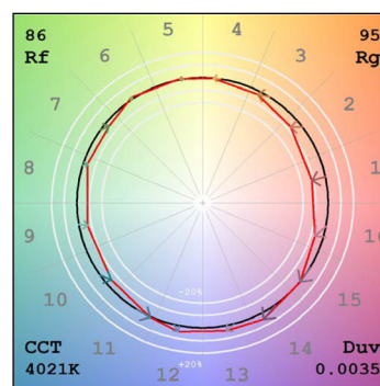
TM-30 Spectrum
