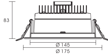
12W 6 inch model Cut out: 150 -165mm
