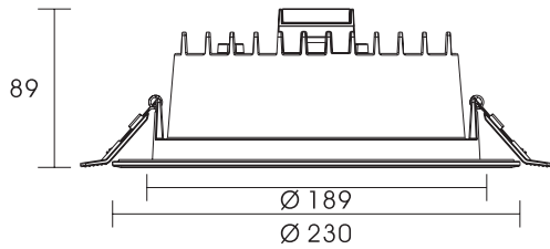
22W & 32W 8 inch models Cut out: 195-215mm
